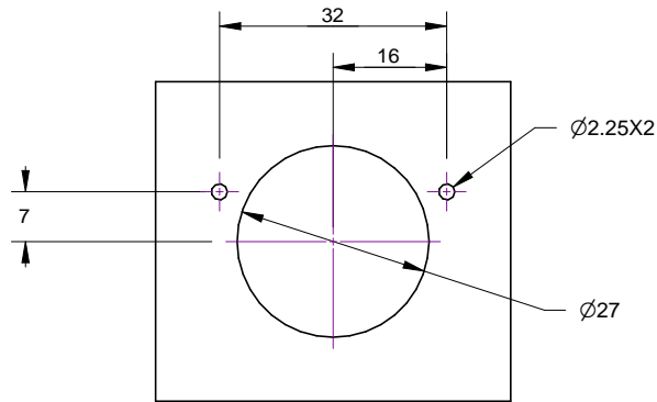
Panel Cutout
